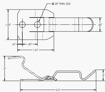
Dura-Clip® Fastener
