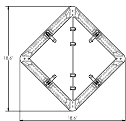
Installation Orientation
