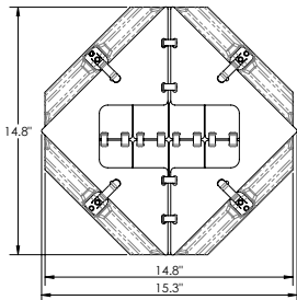
Installation Orientation
