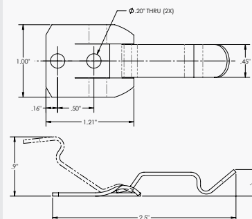
Dura-Clip® Fastener
