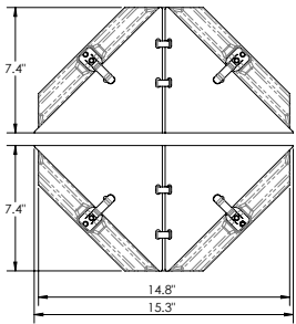
Installation Orientation
