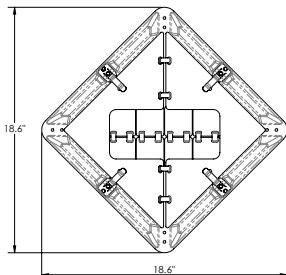
Installation Orientation
